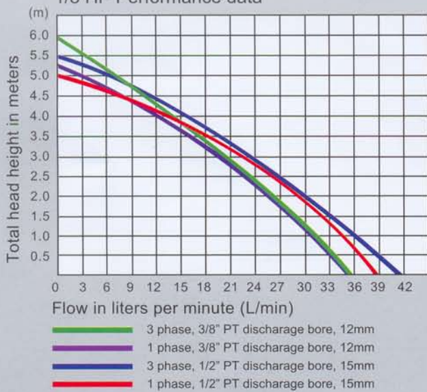
1/8 HP Performance data
