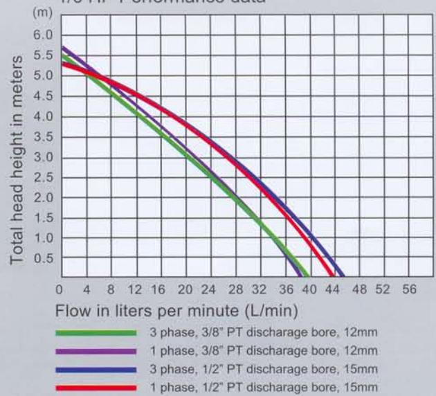
1/6 HP Performance data
